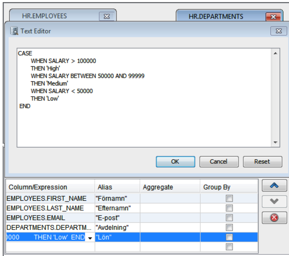
Figure: The Columns tab with the multi-line editor for a custom expression
