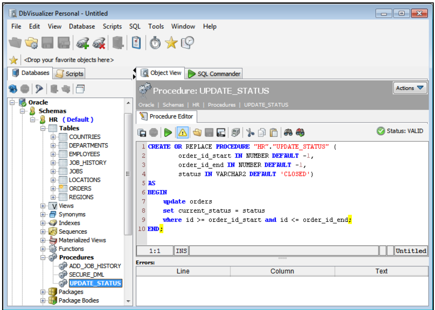
Figure: Compiling procedure with successful result
