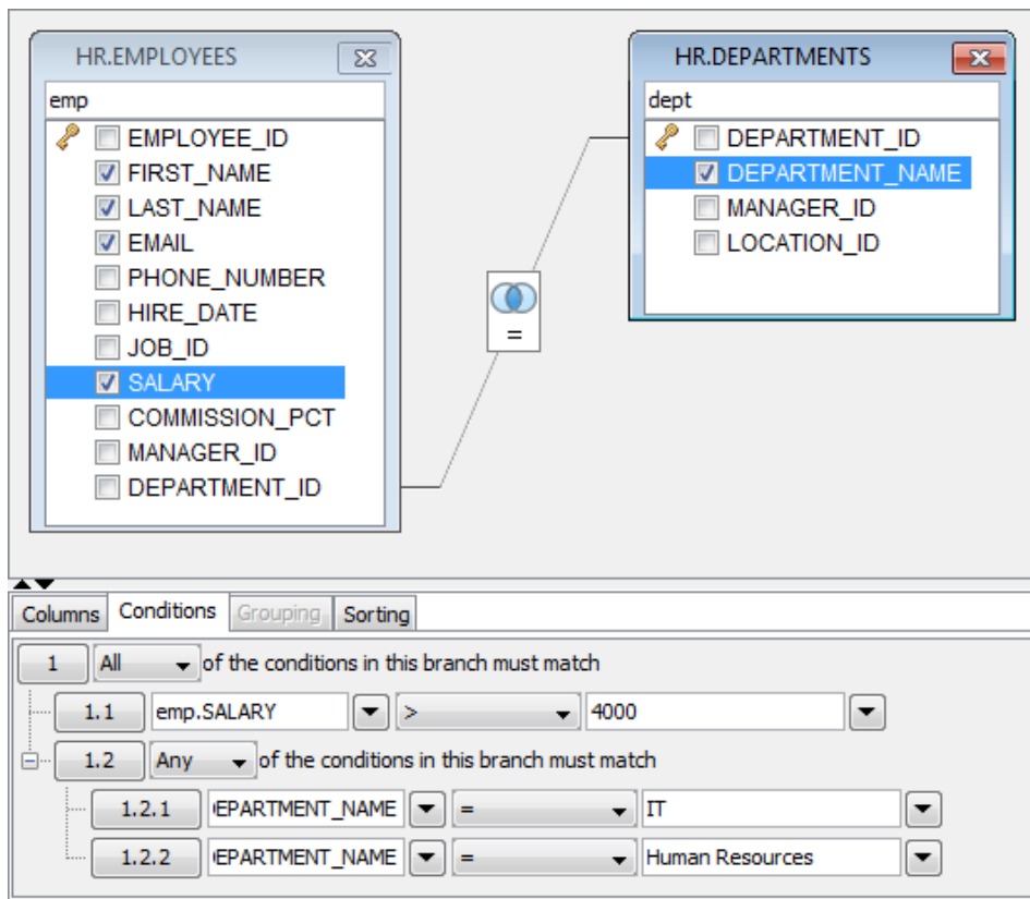
Figure: Condition settings
