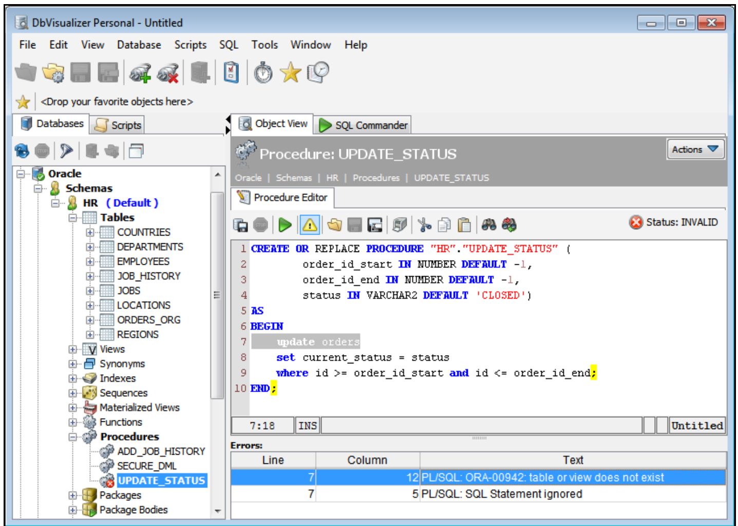
Figure: Compiling procedure with errors
