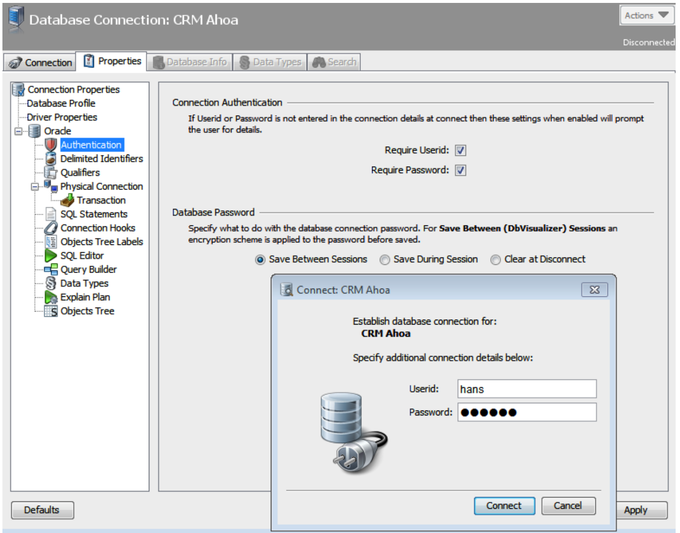
Figure: Dialog asking for Userid and Password as a result of having Require Userid and Password settings enabled
