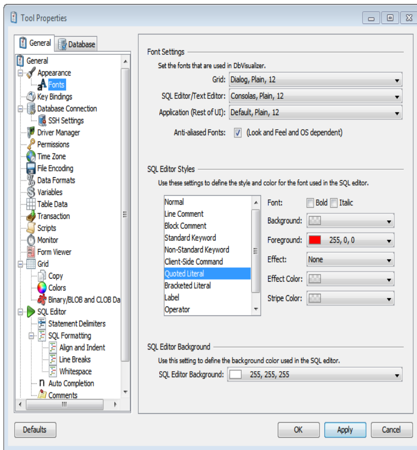
Figure: Fonts settings, with SQL Editor Styles and SQL Editor Background
