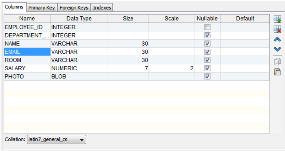
Figure: Collation control
