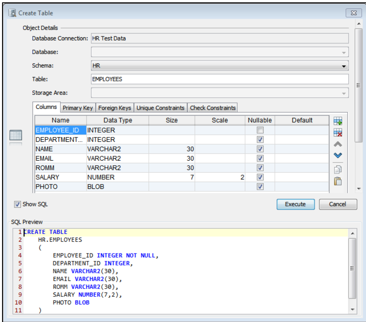
Figure: The Create Table assistant
