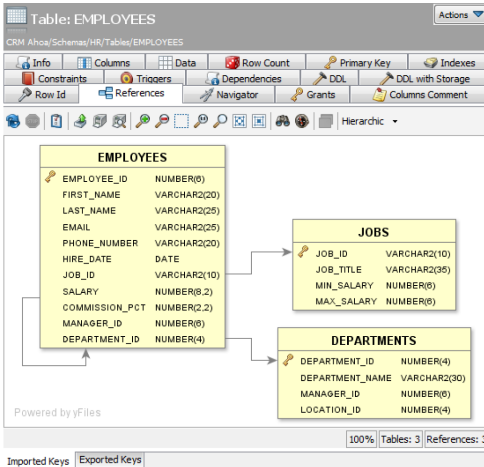
Figure: The references graph showing imported keys for a table
