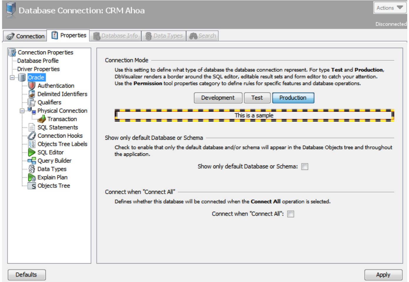
Figure: Connection Properties
