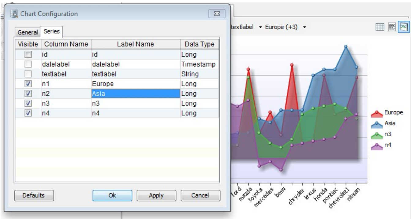
Figure: The Series tab in the Chart Preferences
