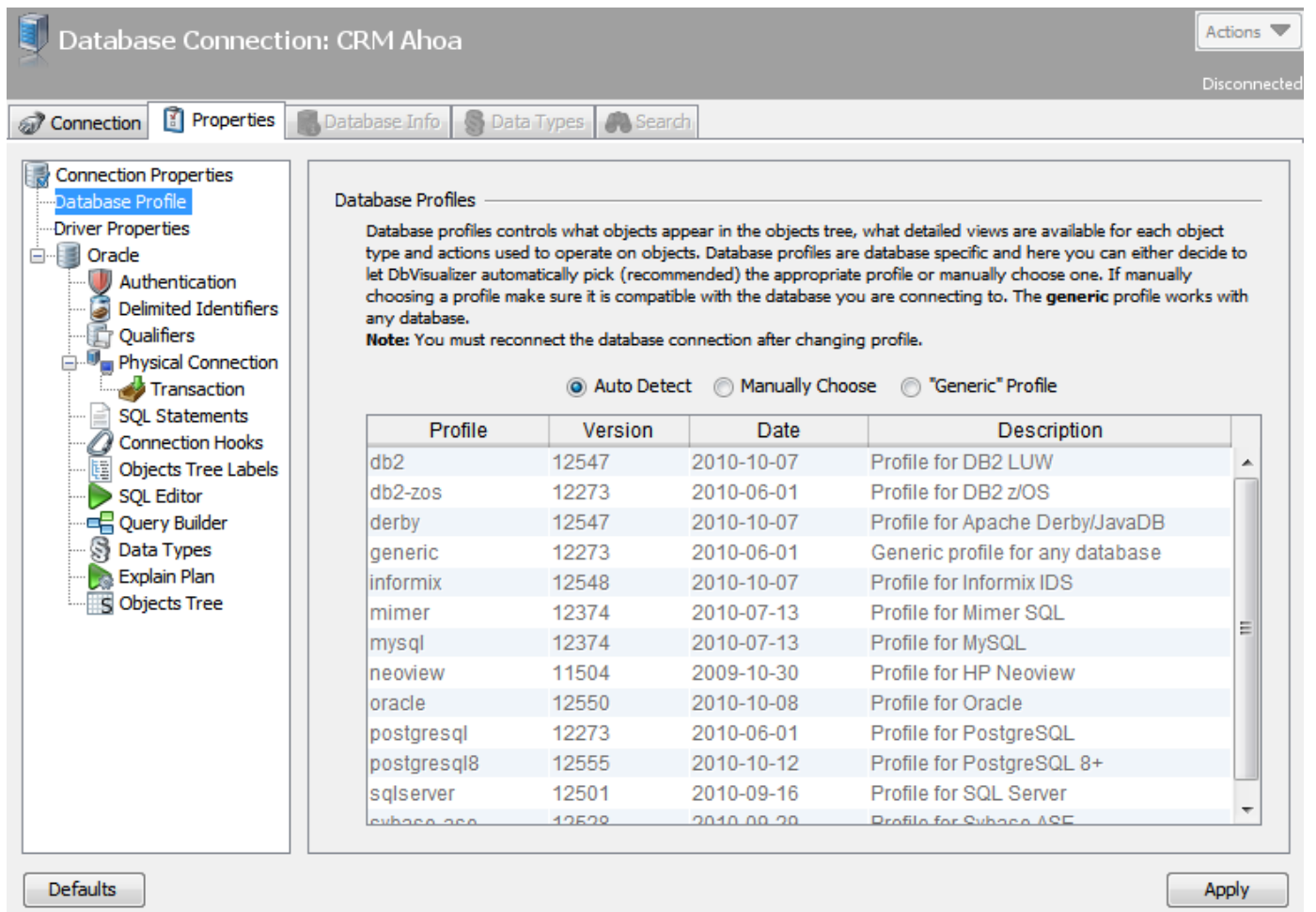
Figure: Database Profile category for a database connection
