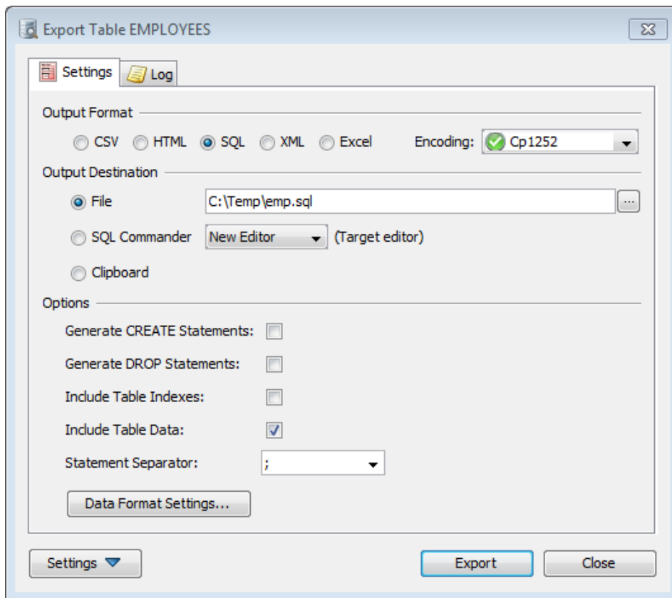
Figure: The Export Table dialog
