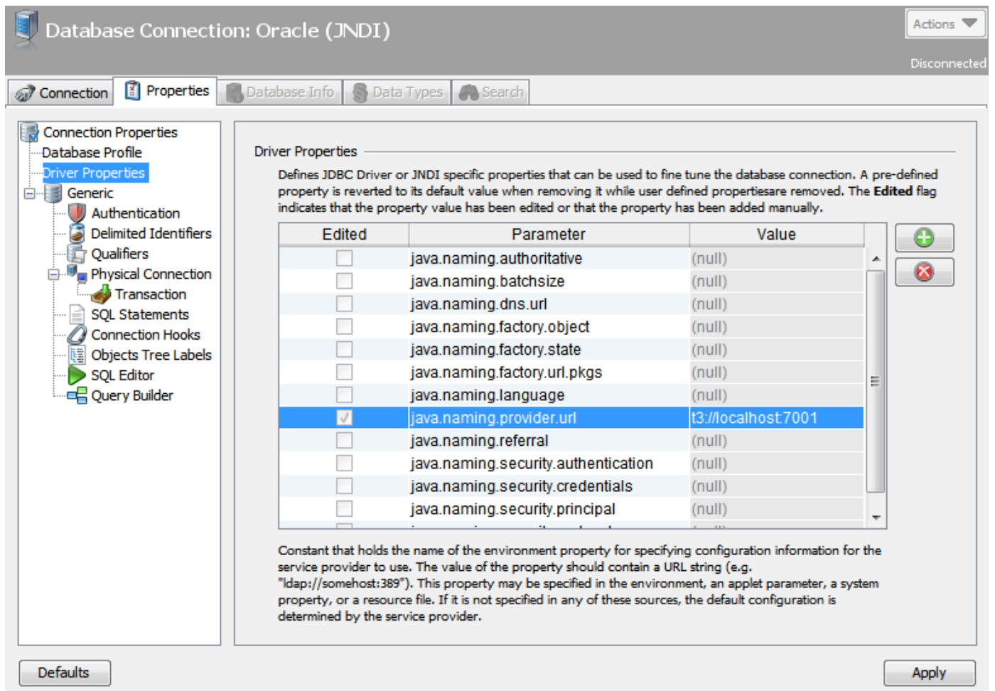
Figure: Driver Properties for JNDI lookup
