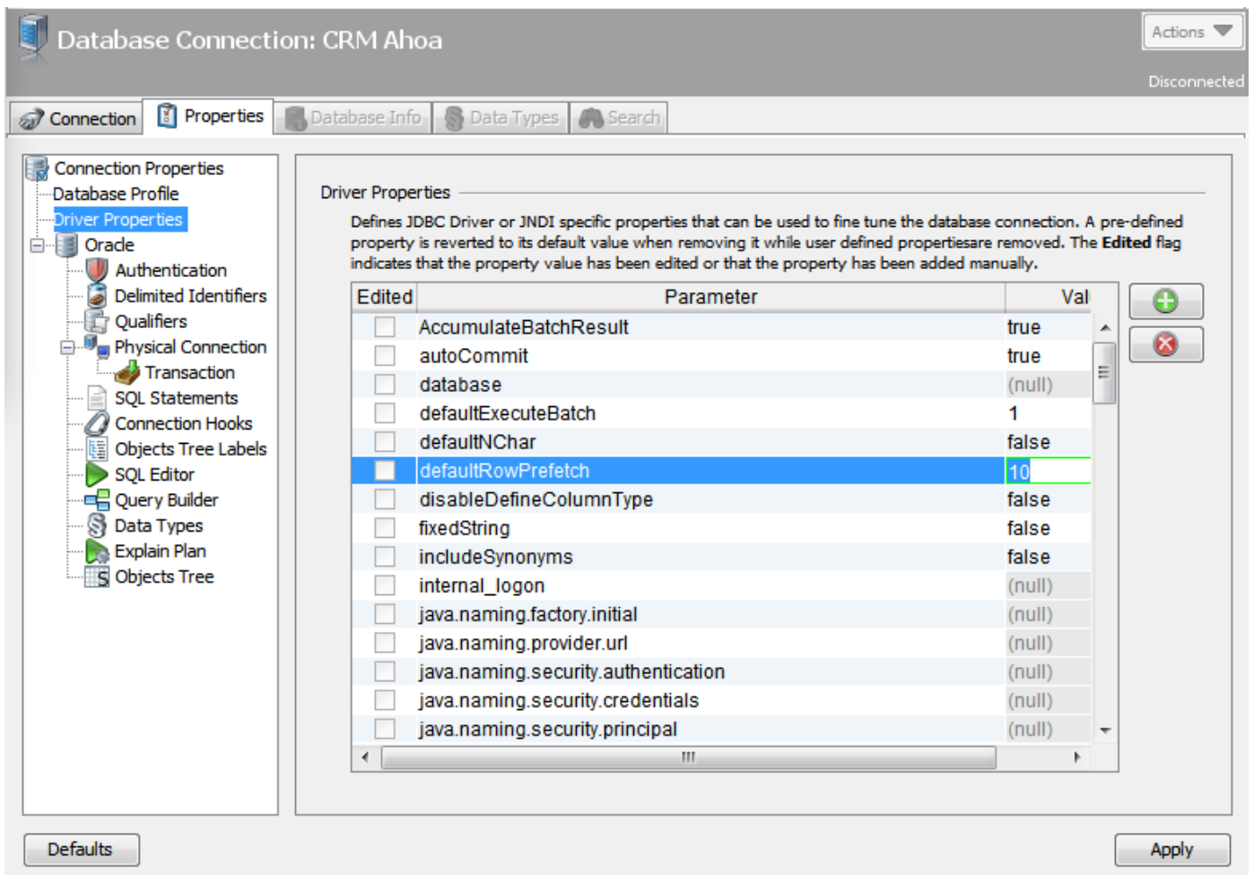
Figure: Driver Properties for JDBC Driver
