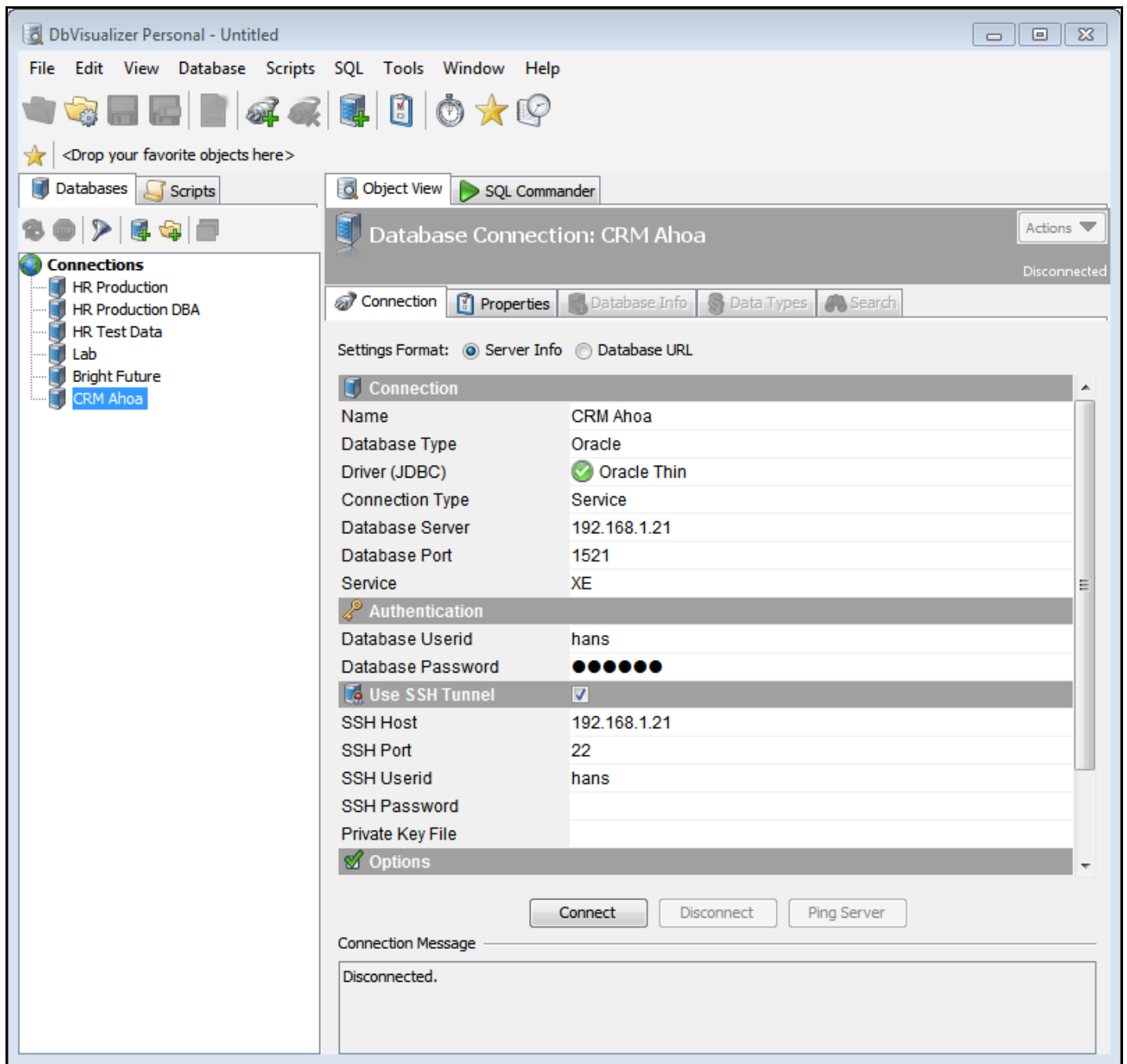
Figure: Database Connection Using an SSH Tunnel
