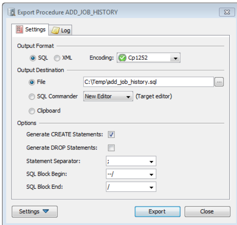
Figure: The Export Procedure dialog
